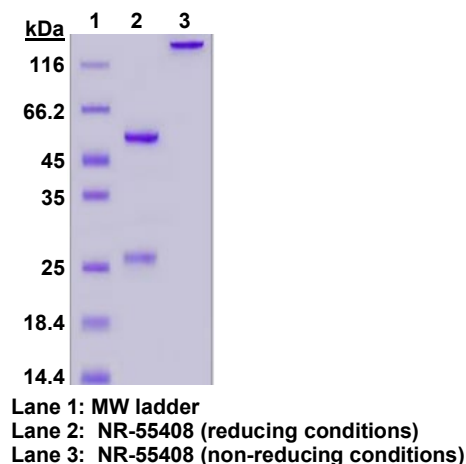
Figure 1: SDS-PAGE Analysis
