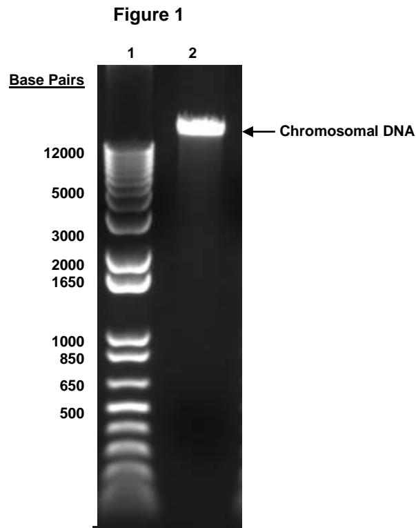
Lane 1: Invitrogen™ TrackIt 1 Kb Plus DNA Ladder™ Lane 2: 200 ng of NR-4606
