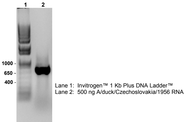
Figure 1: RT-PCR Amplification of Genomic RNA from Influenza A Virus, A/duck/Czechoslovakia/1956 (H4N6)
