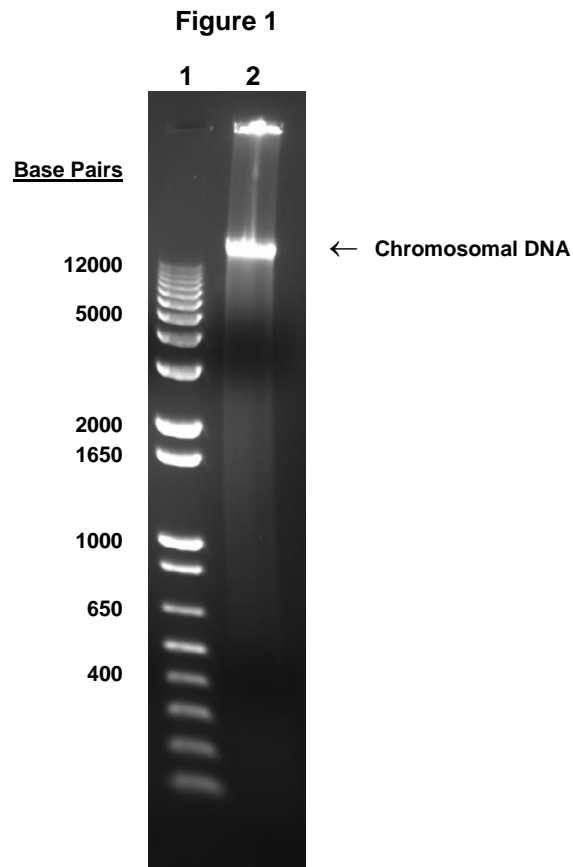
Lane 1: Invitrogen™ TrackIt™ 1 Kb Plus DNA Ladder Lane 2: 200 ng of NR-3020
