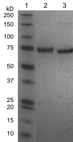
Figure 1: SDS-PAGE
