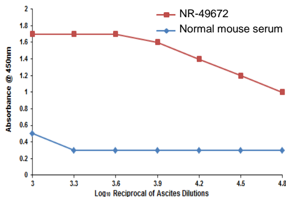
Figure 1 – ELISA
