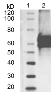
Figure 2 – Western Blot
