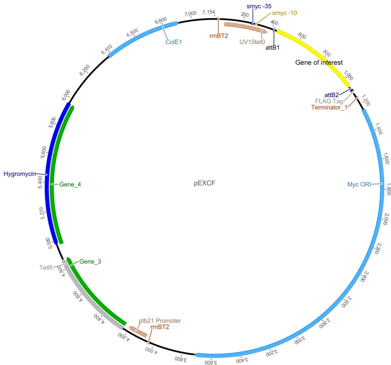
Figure 1: Plasmid Map of pEXCF
