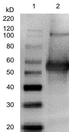
Figure 2: Western Blot with Polyclonal Anti-N7 NA
