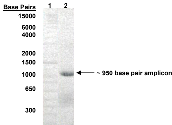
Figure 1: Functional Activity by RT-PCR Amplification
