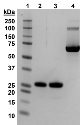
Figure 1: SDS-PAGE of Mpt64
