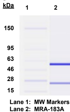
Figure 1: Agilent Protein 230 Analysis
