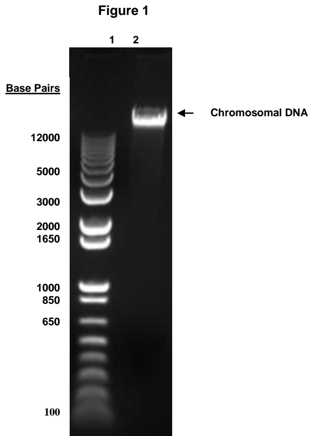
Lane 1: Invitrogen™ TrackIt 1 Kb Plus DNA Ladder™ Lane 2: 200 ng of NR-4585
