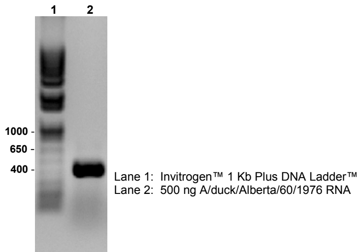
Figure 1: RT-PCR Amplification of Genomic RNA from Influenza A Virus, A/duck/Alberta/60/1976 (H12N5)
