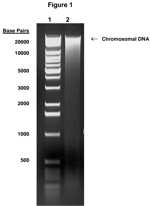
Lane 1: Invitrogen™ 1 Kb DNA Extension Ladder Lane 2: 100 ng of NR-2532
