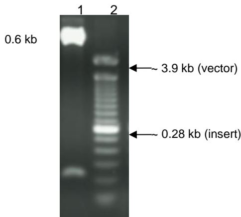
Figure 1: Restriction Enzyme Digestion of Mucin Gene Fragment
