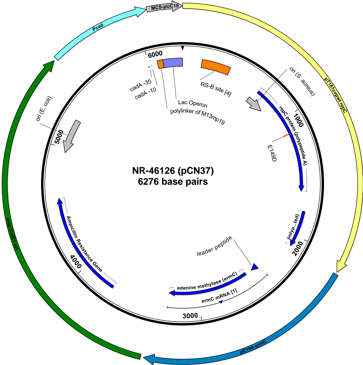
Figure 2: Shuttle Vector pCN37
