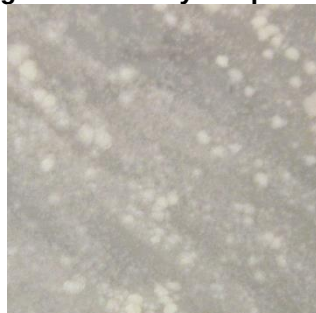
Figure 1: Colony Morphology
