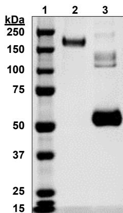
Figure 1: SDS-PAGE Analysis
