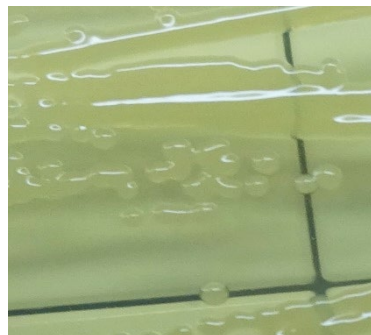
Figure 1: Colony Morphology
